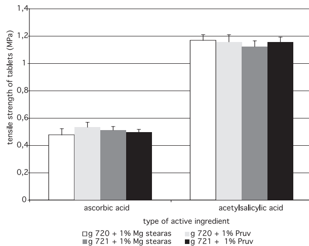
Fig. 5. Tensile strength of tablets at the compression force of 10kN: galen IQ 720 and 721 with active ingredients g 720 – galen IQ 720, g 721 – galenIQ 721, Mg stearas – magnesii stearas
