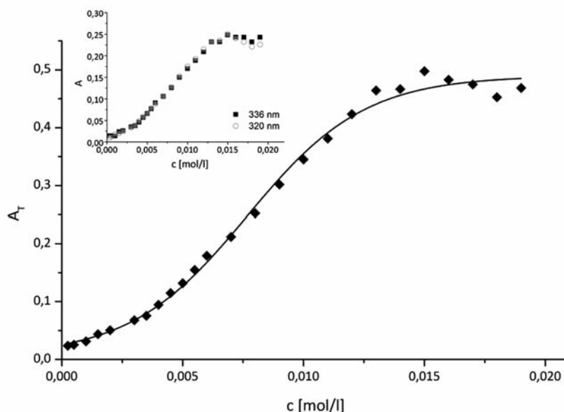
Fig. 3. A_T vs. concentration of (K 1902) in 0.3 mol/l methanol solution profile for pyrene(0.2 \mu\text{mol/l} ) at t = 25^\circ\text{C} . Inset: the pyrene plots of absorbances of two peaks (320 and 336 nm) A versus concentration of surfactant K 1902 in solvent systems
